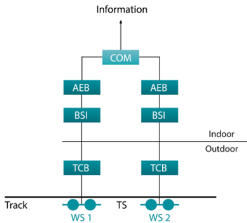
Frauscher Advanced Counter FAdC
