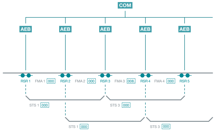
STS overlay the existing track sections
