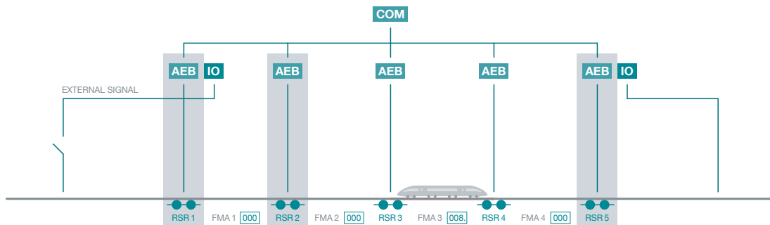
CHC Active counting heads at traversed sections
